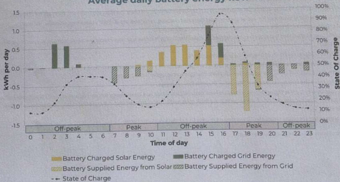
Average daily battery energy flow
