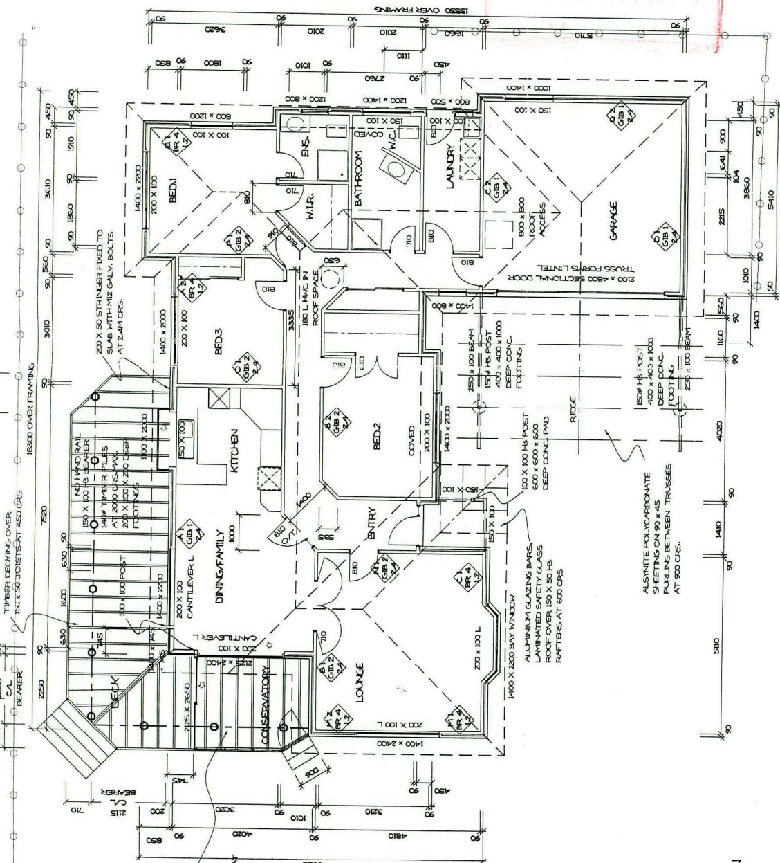
FLOOR PLAN 1:100
