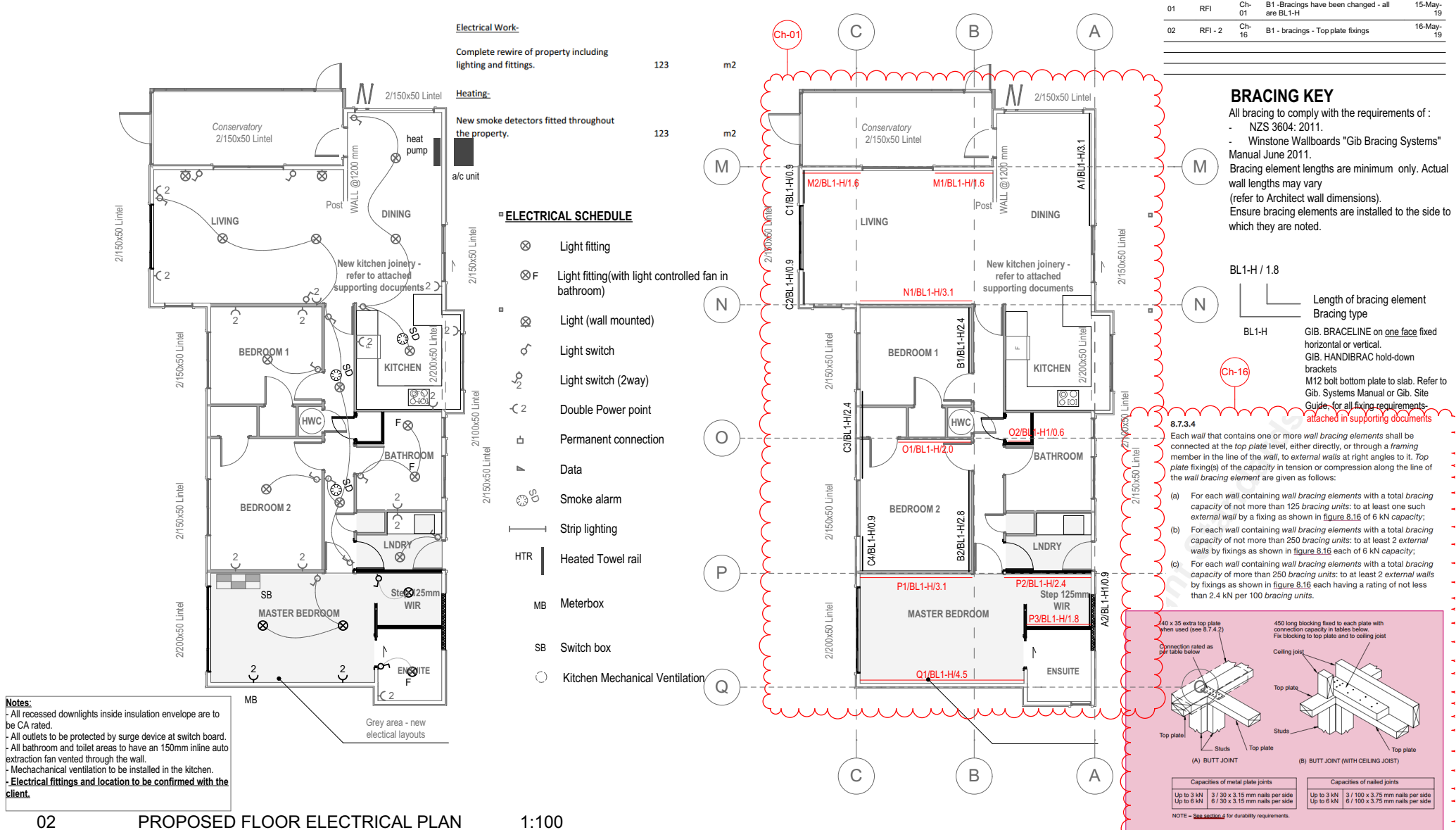
02 PROPOSED FLOOR ELECTRICAL PLAN 1:100
